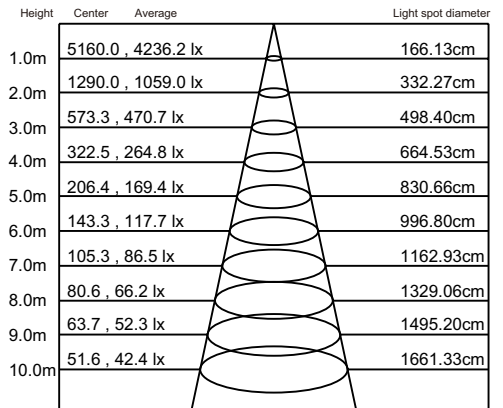
Average illumination test chart
