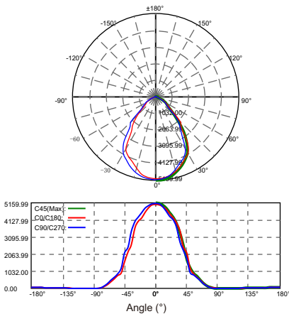
Lighting distribution curve
